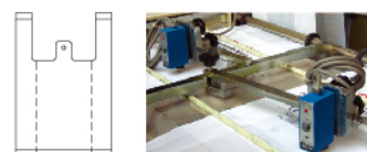
Double photocell
