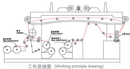
工作原理图 (Working principle drawing)
